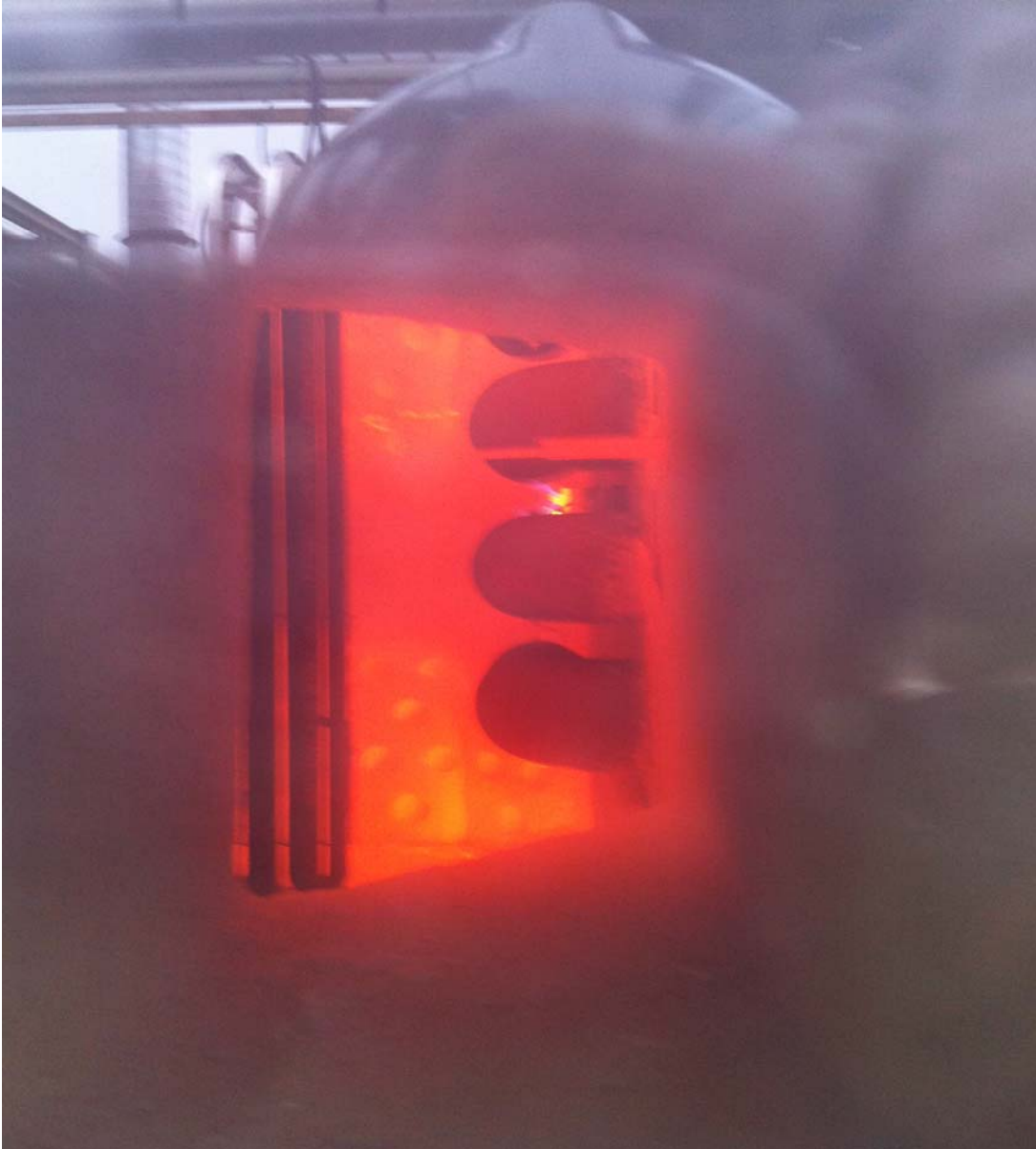
Figure 7. Flameless Firing. View from behind FNG.
