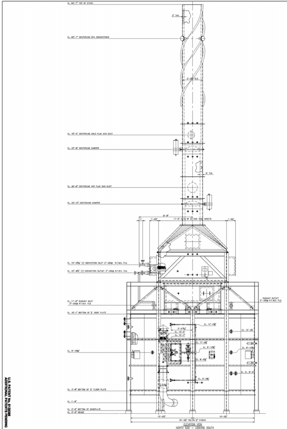
Figure 1. Elevation View of Heater
